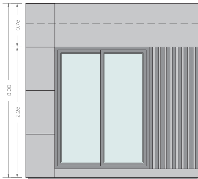
ALZADO PRINCIPAL
