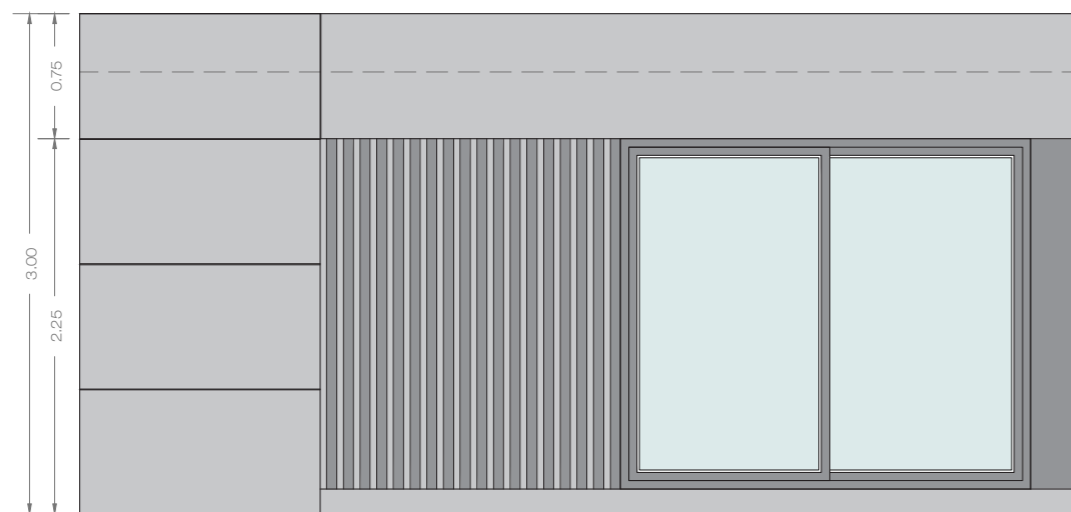
ALZADO PRINCIPAL
