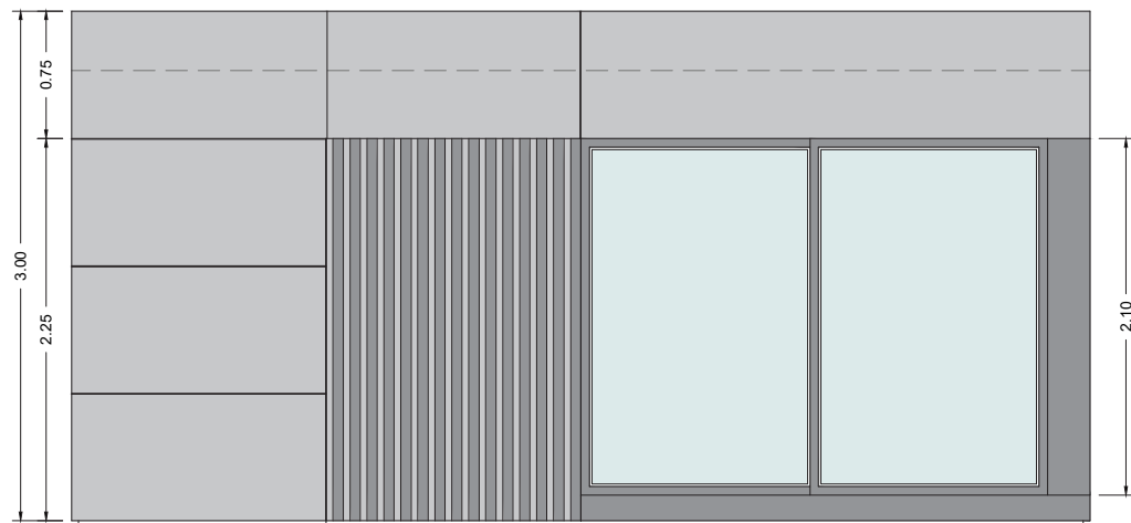
Alzado principal
