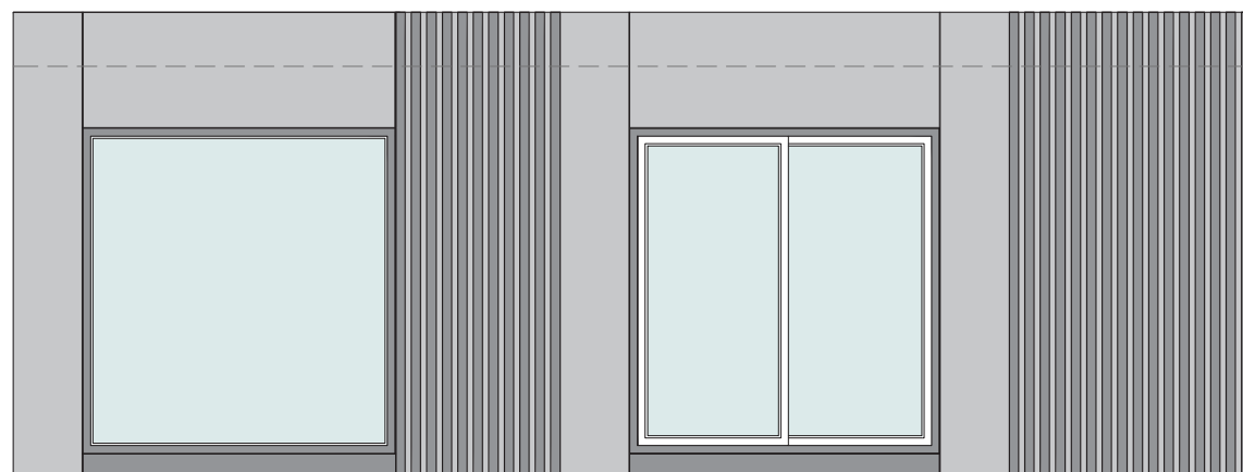
ALZADO PRINCIPAL
