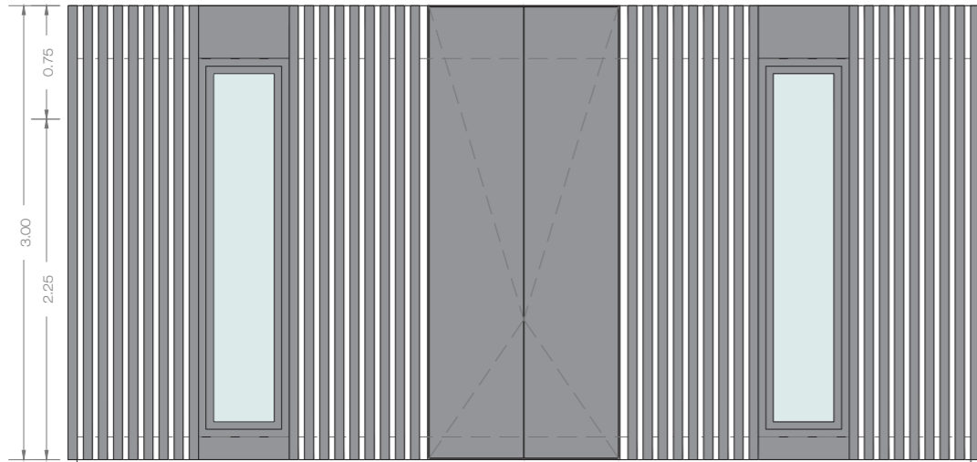
ALZADO PRINCIPAL
